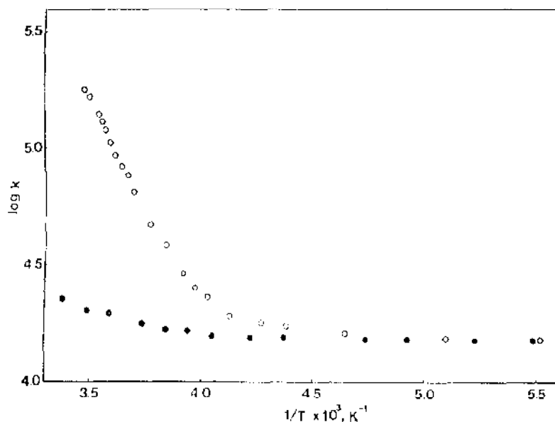
Fig. 5. Contrast in (^2E_g)\text{Cr}(\text{NH}_3)_6^{3+} lifetimes in fluid DMF/ \text{CHCl}_3 solutions (open circles) and in the crystalline solid [\text{Cr}(\text{NH}_3)_6]\text{Cl}_3 doped into [\text{Ru}(\text{NH}_3)_6]\text{Cl}_3 with Cr:Ru = 1:30; (closed circles). From [79].
