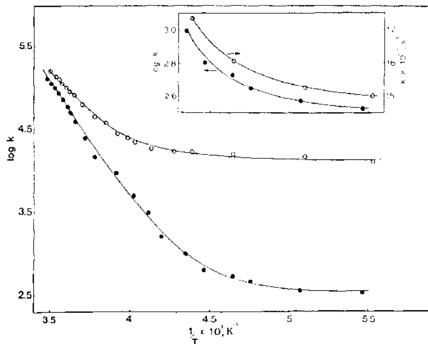
Fig. 4. Temperature dependencies of the {}^2E_g lifetimes for [\text{Cr}(\text{NH}_3)_6](\text{ClO}_4)_3 (open circles) and [\text{Cr}(\text{ND}_3)_6](\text{ClO}_4)_3 (closed circles) in \text{DMF}-\text{CHCl}_3 solution. Inset expands the rate constant scale in the low temperature regime. From [79].
