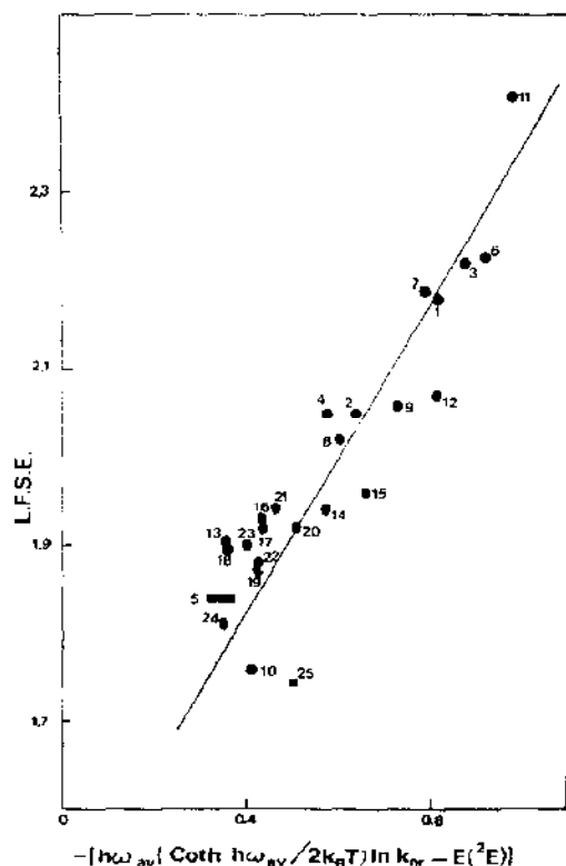
Fig. 10. Correlation of {}^2E excited state lifetimes of \text{Cr}^{\text{III}} amine complexes in aqueous solution and LFSE based on a simple strong coupling surface crossing model using \hbar\omega_{\text{ave}} = 400 \text{ cm}^{-1} and the energy of lowest LF absorption maximum ( {}^4T_{2g} in O_h or the mean of {}^4E and {}^4B components in lower symmetry) has been used for LFSE (energies in \text{cm}^{-1}/10^4 ). The correlation is based on eqn. 13 with \lambda \gg \Delta E , E_d \sim \lambda/4 - \Delta E/2 , \hbar\omega_{\text{ave}} \sim 400 \text{ cm}^{-1} , and
