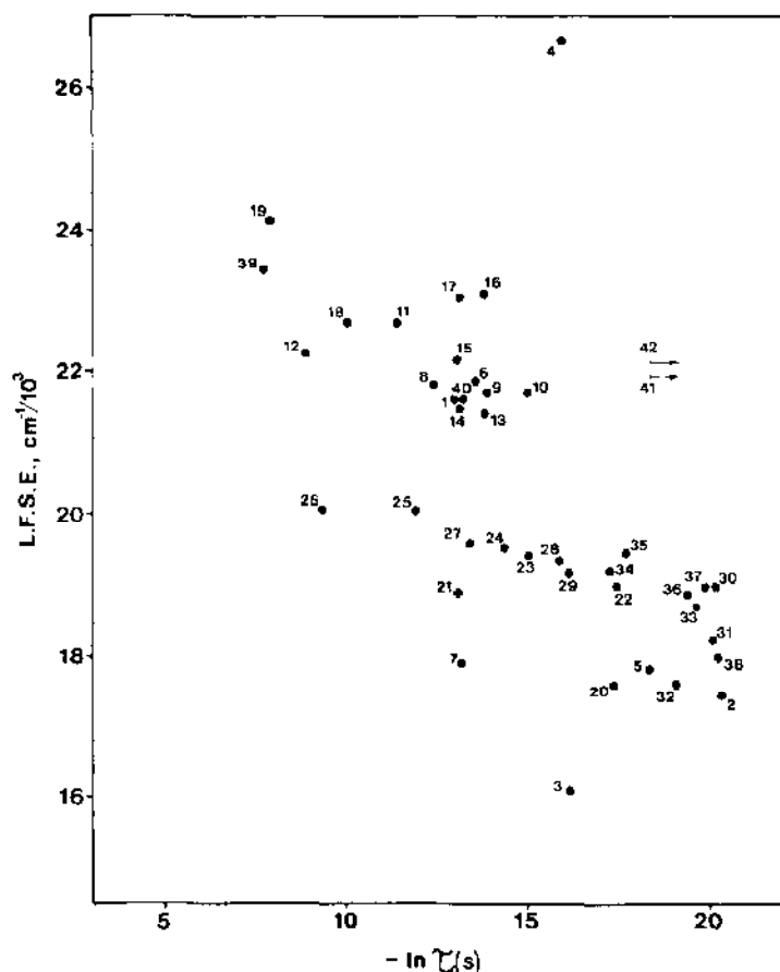
Fig. 9. Correlation of ligand field stabilization energy (LFSE) with the mean ^2E decay time (in aqueous solution at 25°C except as indicated) for several Cr(III) complexes. Energy of lowest LF absorption used for LFSE. Data from Tables 3, 4, 6 and 7. Key to points: 1, \text{Cr}(\text{NH}_3)_6^{3+} . 2, \text{Cr}(\text{OH}_2)_6^{3+} . 3, \text{Cr}(\text{urea})_6^{3+} . 4, \text{Cr}(\text{CN})_6^{3-} . 5, \text{Cr}(\text{NCS})_6^{3-} . 6, \text{Cr}(\text{en})_3^{3+} . 7, \text{Cr}(\text{acac})_3 . 8, \text{Cr}(\text{sep})_3^{3+} (in DMF). 9, \text{Cr}(\text{chda})_3^{3+} (in DMF). 10, \text{Cr}(\text{dien})_2^{3+} (in DMF). 11, \text{Cr}([9]\text{aneN}_3)_2^{3+} . 12, \text{trans-Cr}([14]\text{aneN}_4)(\text{NH}_3)_2^{3+} . 13, \text{cis-Cr}([14]\text{aneN}_4)(\text{NH}_3)_2^{3+} . 14, \text{cis-Cr}([14]\text{aneN}_4)\text{en}^{3+} . 15, \text{Cr}(\text{NH}_3)_5\text{CN}^{2+} . 16, \text{trans-Cr}(\text{en})_2(\text{CN})_2^- . 17, \text{cis-Cr}(\text{en})_2(\text{CN})_2^- . 18, \text{trans-Cr}(\text{NH}_3)_4(\text{CN})_2^- . 19, \text{trans-Cr}([14]\text{aneN}_4)(\text{CN})_2^- . 20, \text{trans-Cr}([14]\text{aneN}_4)\text{Cl}_2^- . 21, \text{trans-Cr}(\text{en})_2\text{F}_2^+ . 22, \text{trans-Cr}(\text{en})_2(\text{OH}_2)\text{F}_2^+ . 23, \text{trans-Cr}(\text{en})_2(\text{NCS})\text{F}^+ . 24, \text{trans-Cr}(\text{NH}_3)_4(\text{NCS})_2^- . 25, \text{trans-Cr}(\text{en})_2(\text{NCS})_2^+ . 26, \text{trans-Cr}([14]\text{aneN}_4)(\text{NCS})_2^- . 27, \text{trans-Cr}(\text{tn})_2(\text{NCS})_2^+ . 28, \text{trans-Cr}(\text{en})_2(\text{OH}_2)\text{NCS}^{2+} . 29, \text{trans-Cr}(\text{tn})_2(\text{OH}_2)\text{NCS}^{2+} . 30, \text{trans-Cr}(\text{NH}_3)_4(\text{OH}_2)\text{NCS}^{2+} . 31, \text{trans-Cr}(\text{en})_2(\text{NCS})\text{Br}^- . 32, \text{trans-Cr}(\text{NH}_3)_2(\text{NCS})_4^- . 33, \text{trans-Cr}(\text{tn})_2(\text{OH}_2)_2^{3+} . 34, \text{cis-Cr}(\text{tn})_2(\text{OH}_2)\text{NCS}^{2+} . 35, \text{cis-Cr}(\text{en})_2(\text{OH}_2)\text{NCS}^{2+} . 36, \text{cis-Cr}(\text{tn})_2(\text{OH}_2)_2^{3+} . 37, \text{cis-Cr}(\text{en})_2(\text{OH}_2)_2^{3+} . 38, \text{cis-Cr}(\text{tn})_2(\text{OH}_2)(\text{Cl})_2^{2+} . 39, \text{trans-(ms-(5,12)-Me}_6[14]\text{aneN}_4)(\text{CN})_2^- . 40, \text{cis-Cr}(\text{rac-(5,12)-Me}_6[14]\text{aneN}_4)(\text{CN})_2^- . 41, (\text{Cr}(\text{sar}))^{3+} (upper limit for \tau ). 42, \text{Cr}(\text{diansar})^{3+} (upper limit for \tau ).
