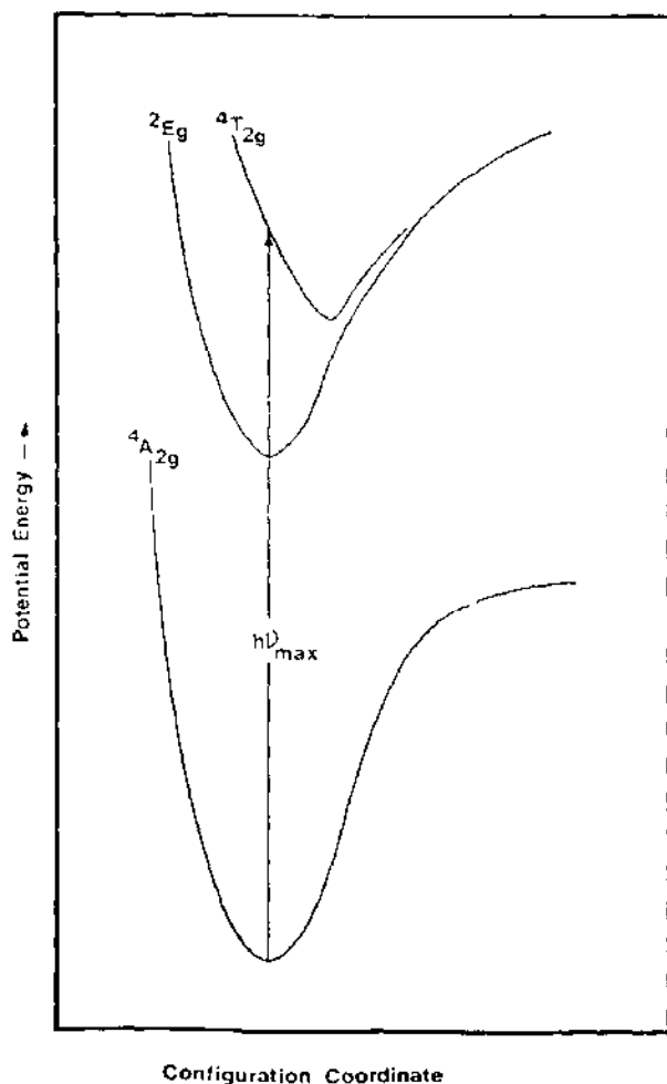
Fig. 3. Qualitative potential energy surfaces for \text{Cr}(\text{NH}_3)_6^{3+} allowing for a substitutional reaction channel.
